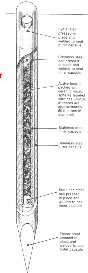
137 Cs Radioactive Seed
