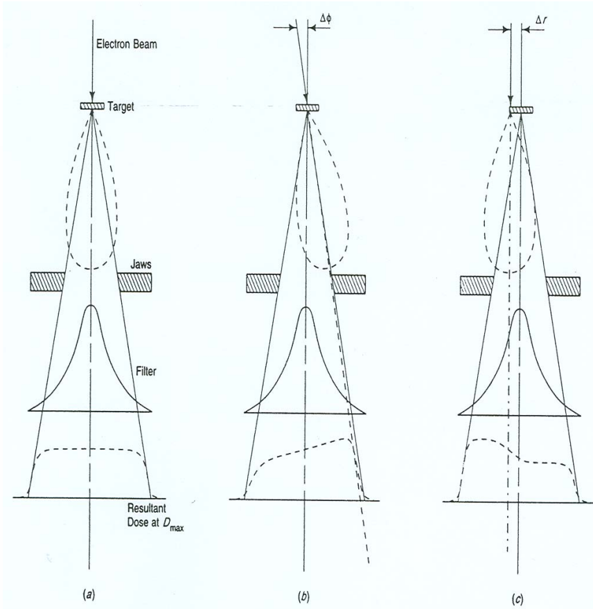
Flattened X-ray field distributions. (a) Symmetrical, electron beam axial at X-ray Target; (b) asymmetrical, electron beam tilted at X-ray target; and (c) asymmetrical, electron beam displaced at X-ray target. (Courtesy of Ref. 6)
