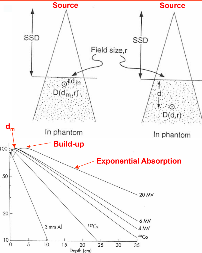
Percent depth dose for 100 cm 2 area X-ray and gamma-ray beams of different energies as a function of depth in water. The SSD is 100 cm for all beams except the 3.0 mm Al (SSD = 15 cm) X-ray beam and the ^{137}\text{Cs} beam (SSD = 35 cm). (From: Hendee WR, Medical Radiation Physics, ed 1, Chicago, 1970, Mosby-Year Book, used with permission.)
