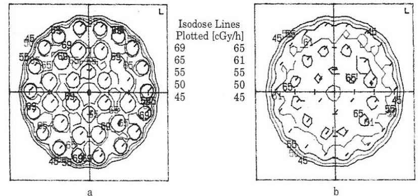
Illustration for the discussion of maximum significant dose and maximum contiguous dose: a) dose distribution through the central seed plane of an eight centimeter long template implant; b) dose distribution 0.5 cm from the plane in a) between seed planes.
