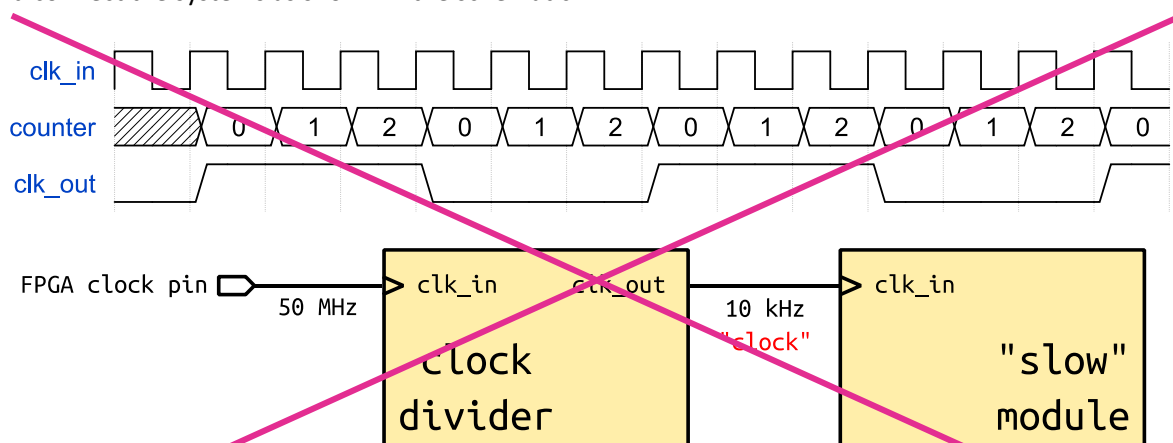
FIGURE 1. Incorrect CLOCK DIVIDER (3x)
