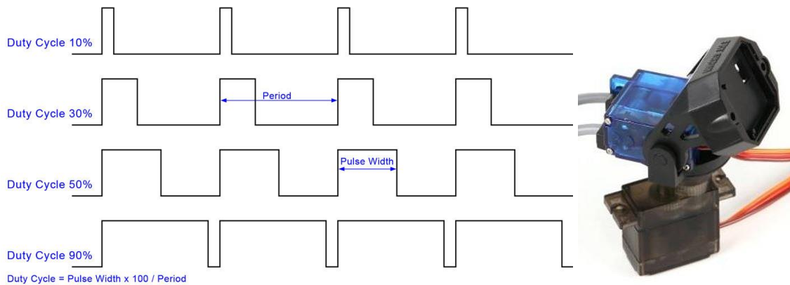
FIGURE 3. PWM WAVEFORMS [1]
