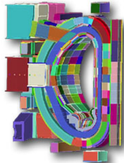
MCNPX-CAD Model for the ITER
