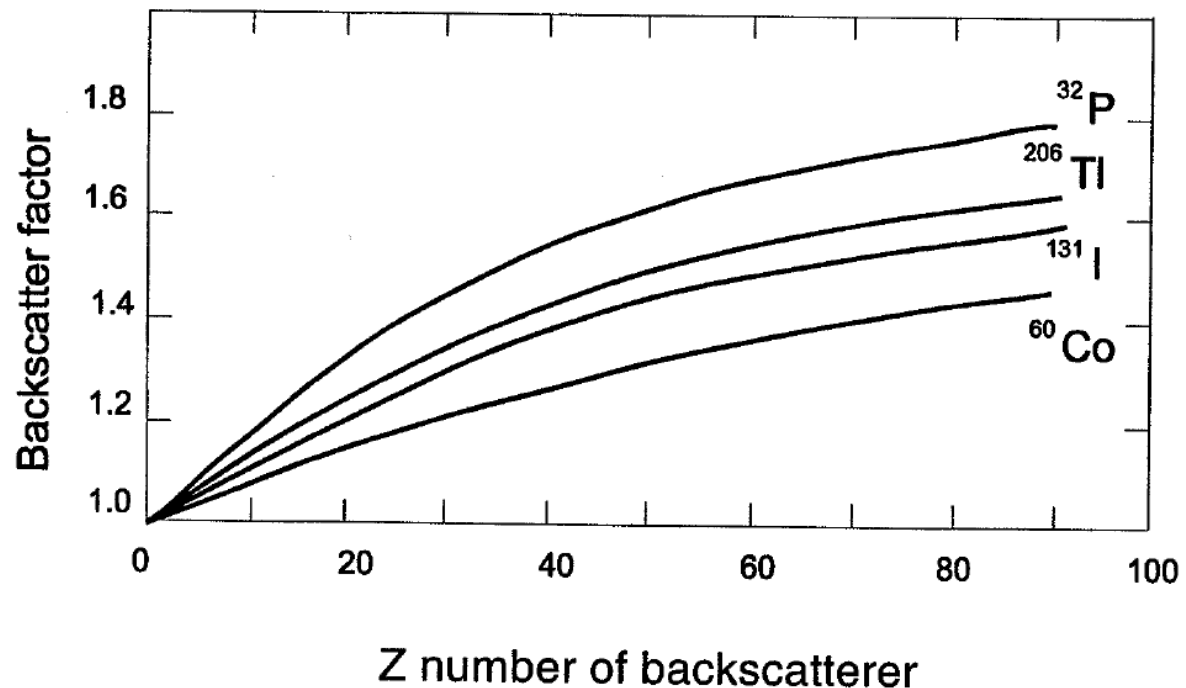
Backscatter factors (relative values), for \beta particles emitted from ^{32}\text{P} (695 keV), ^{206}\text{Tl} (540 keV), ^{131}\text{I} (182 keV), ^{60}\text{Co} (96 keV), as functions of the Z number of the backscatterer. The energies are the averages of each particle spectrum (based on Shapiro, 1972, Figure 4.4).
