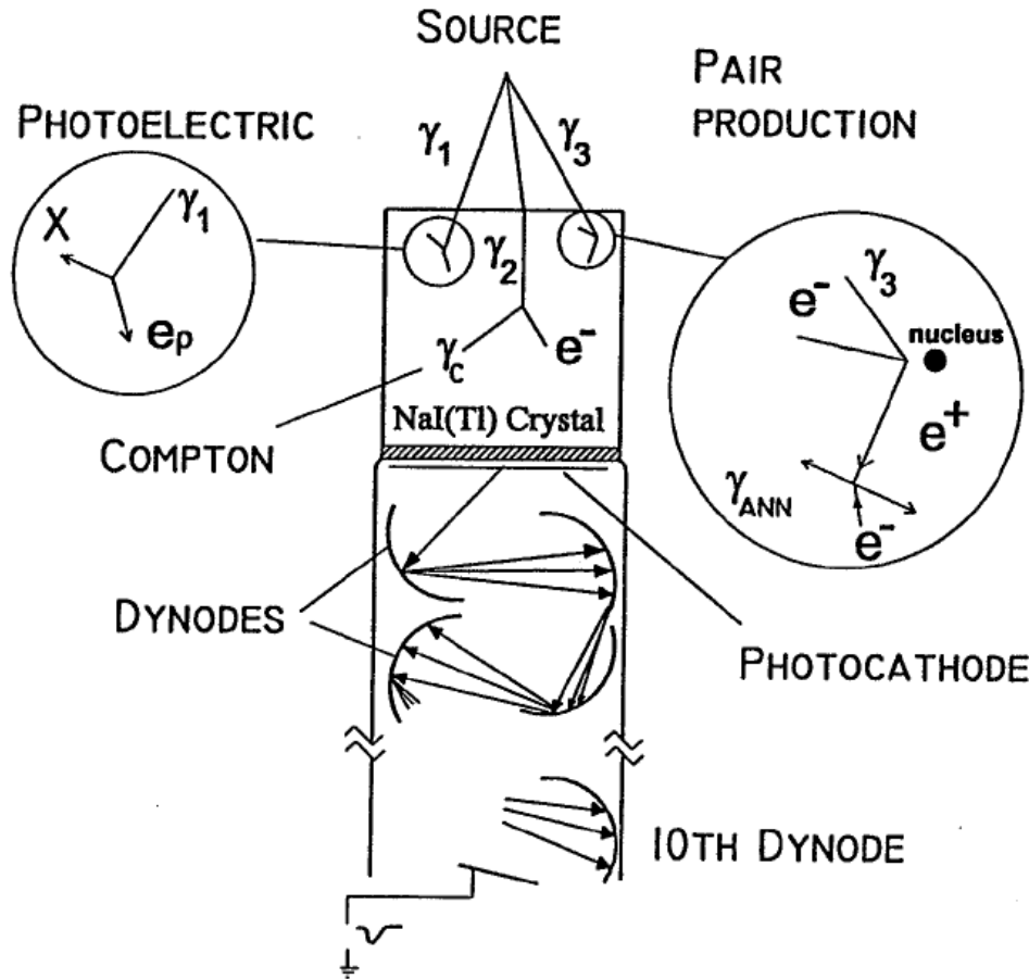
Gamma ray interactions in a NaI(Tl) detector shown with the associated electronics. The photoelectric effect ( \gamma_1 ), Compton scatter ( \gamma_2 ) and pair production ( \gamma_3 ) are illustrated.
