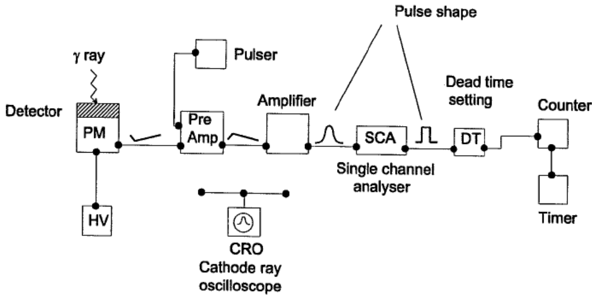
A block diagram of equipment used for the signal processing of pulses due to \gamma rays detected in a NaI(Tl) crystal (see text, Section 4.3.1 for explanations). The pulser and dead time gate (DT) are rarely required for routine work.
