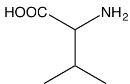
valine
