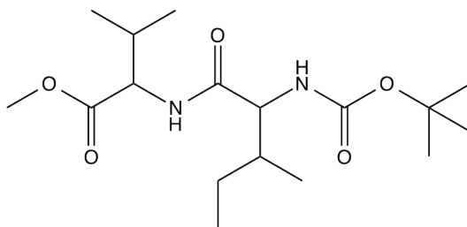
methyl ( tert -butoxycarbonyl)isoleucylvalinate
