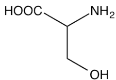
serine
