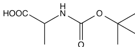
( tert -butoxycarbonyl)alanine
