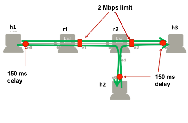
Figure 3: Fairness of TCP connections traversing multiple bottlenecks: wiring and addressing scheme.
