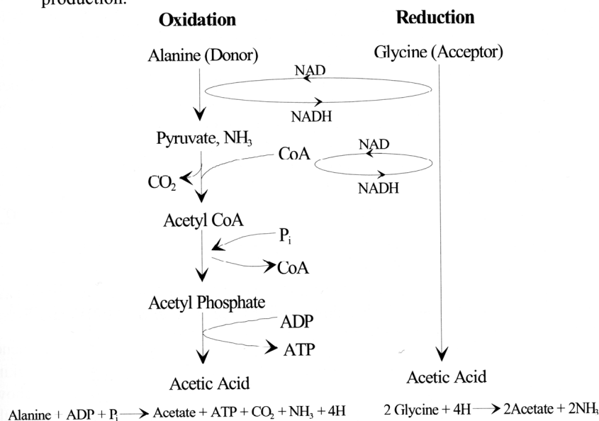
Figure 3.2: Coupled Stickland digestion of alanine and glycine (from Madigan et al. 2000).
