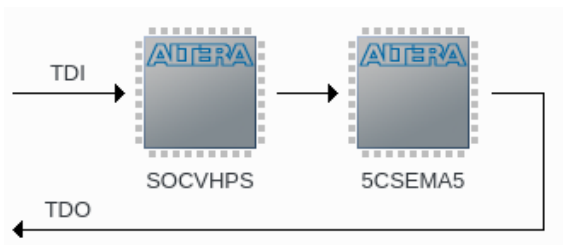
Figure 9-22. JTAG Scan Chain
