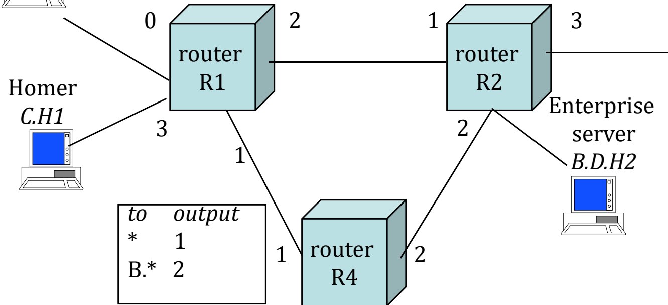
IP Forwarding table
