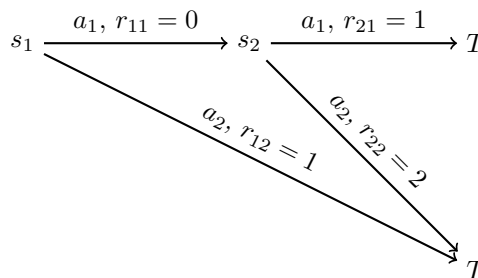
Figure 1: MDP in Exercise 2
