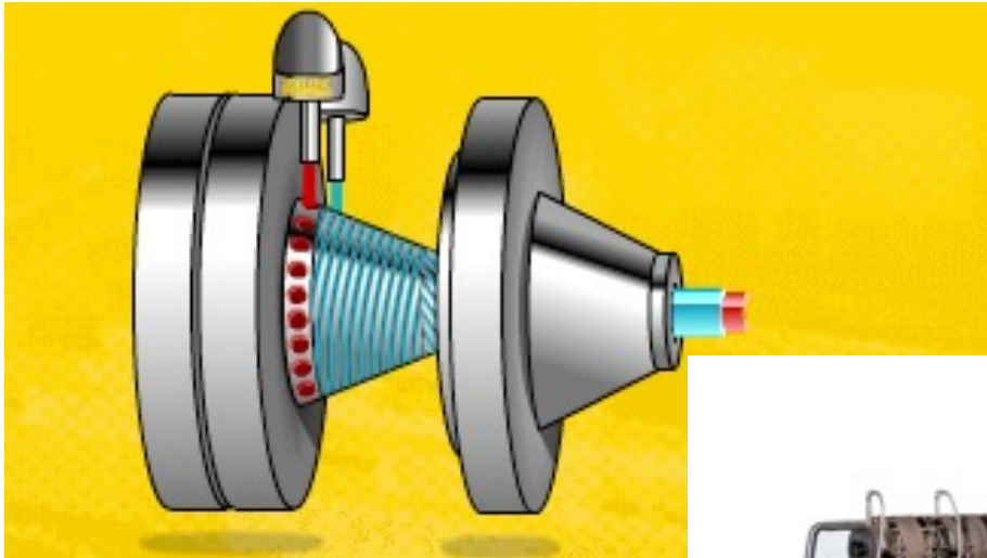
Conical extruder
