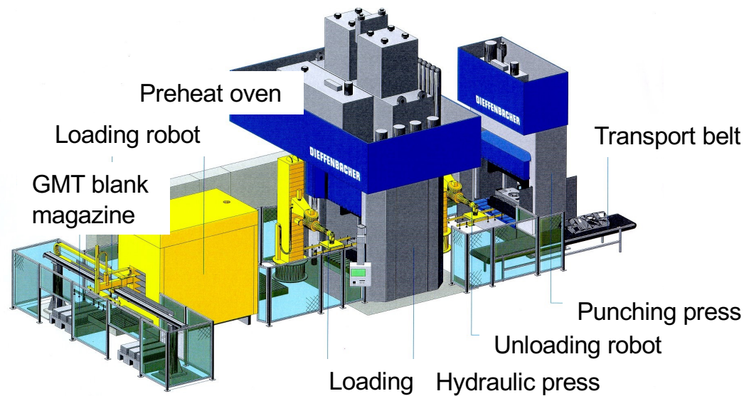
2000 t GMT press for DaimlerChrysler A-class tailgate
