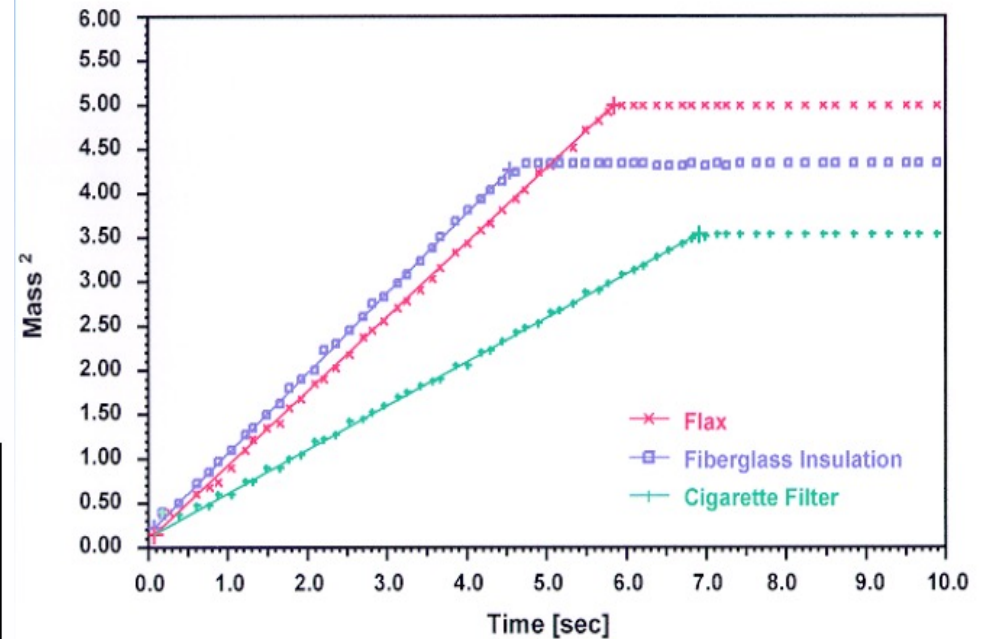
Water Adsorption onto Various Fibrous Materials
