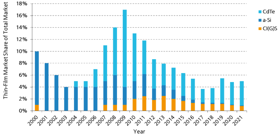
Data: from 2000 to 2009: Navigant; from 2010 to 2021 IHS Markit; from 2022 IEA. Graph: PSE 2022. Date of data: July 2022
