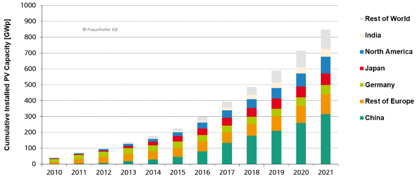
Data: IRENA 2022. Graph: PSE 2022. Date of data: Apr-2022
